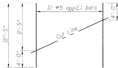
FIELD CUTTING DIAGRAM Order V102(E) full length. Cut as shown and use remainder of bars in opposite face.
