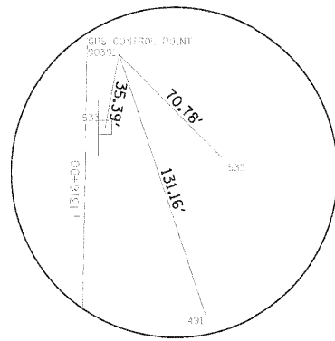
HORIZONTAL CONTROL POINT NO. 90391 IL-92
