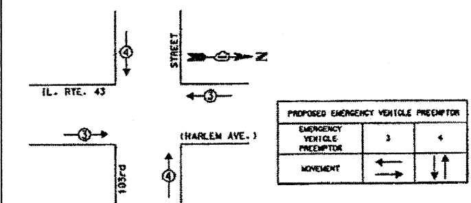
EMERGENCY VEHICLE PREEMPTION SEQUENCE
