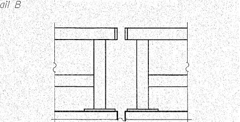
PARAPET RAILING ELEVATION AT EXPANSION JOINT (Two Element Rail Shown)
