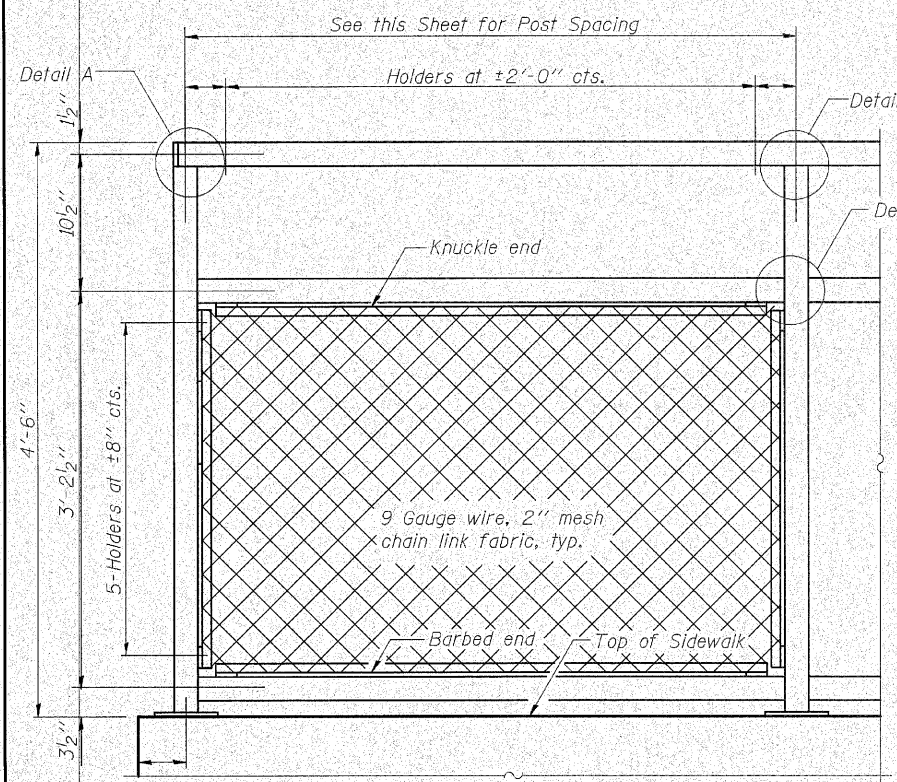
BICYCLE RAILING
