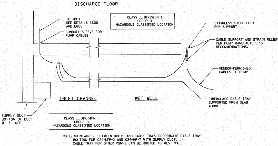
CABLE TRAY DETAIL E601 NTS
