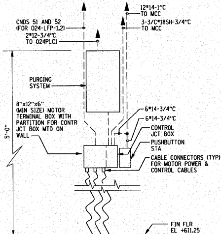
MOTOR TERMINAL BOX DETAIL E605 (TYP. FOR 024-LFP-1, -2) NOT TO SCALE
