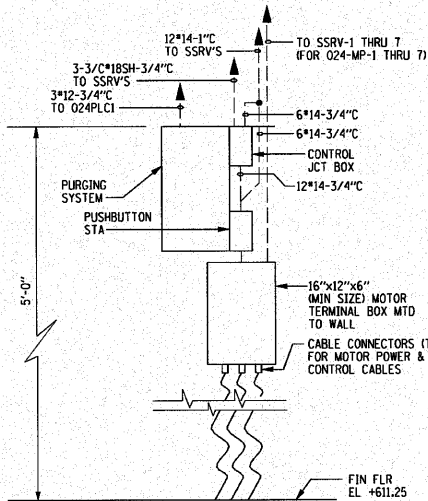
MOTOR TERMINAL BOX DETAIL E600 (TYP. FOR 024-MP-1 THRU MP-7) NOT TO SCALE
