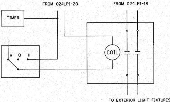
LIGHTING CONTACTOR AND TIMER WIRING DIAGRAM E951 NTS
