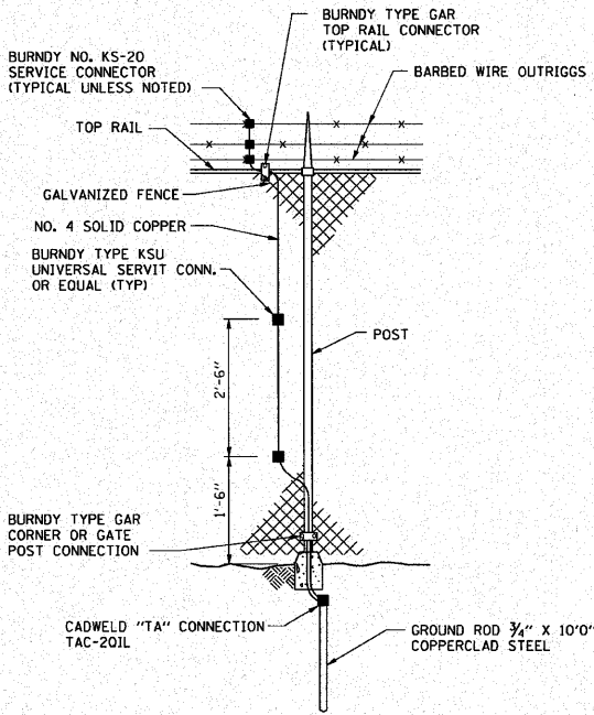
LINE POST GROUNDING E458 NTS
