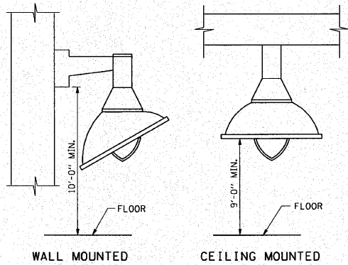
FIXTURE MOUNTING DETAIL E500 NTS
