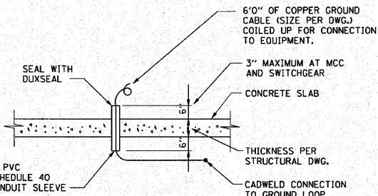
EQUIPMENT GROUND CABLE STUB-UP E452 NTS
