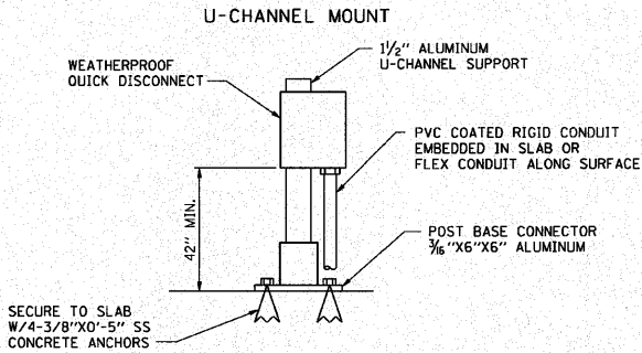
DISCONNECT INSTALLATION E002 NTS
