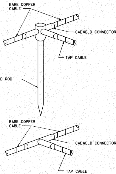
GROUNDING CONNECTION DETAIL E451 NTS
