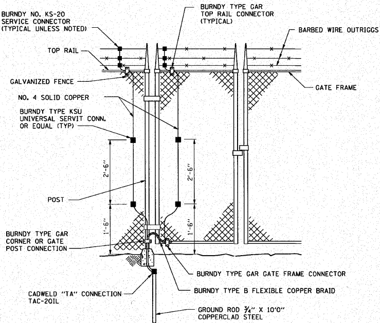
GATE AND HINGE POST GROUNDING E457 NTS
