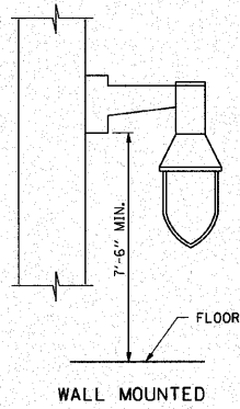
FIXTURE MOUNTING DETAIL E550 NTS
