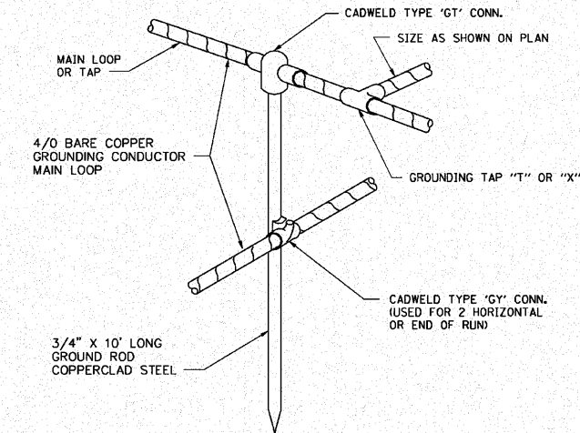
CONDUCTOR TO GROUND ROD CONNECTION DETAIL E451 NTS
