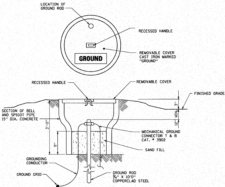
GROUNDING TEST STATION DETAIL E455 NTS
