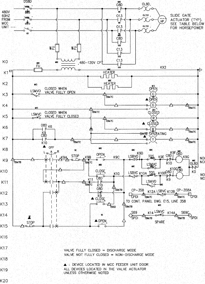
PUMP STATION SLIDE GATE CONTROL SCHEMATIC
