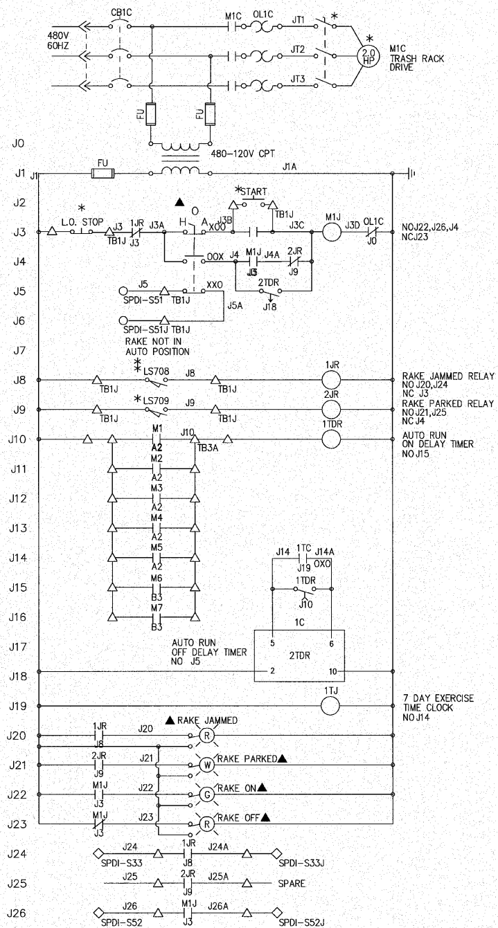
TRASH RACK DRIVE
