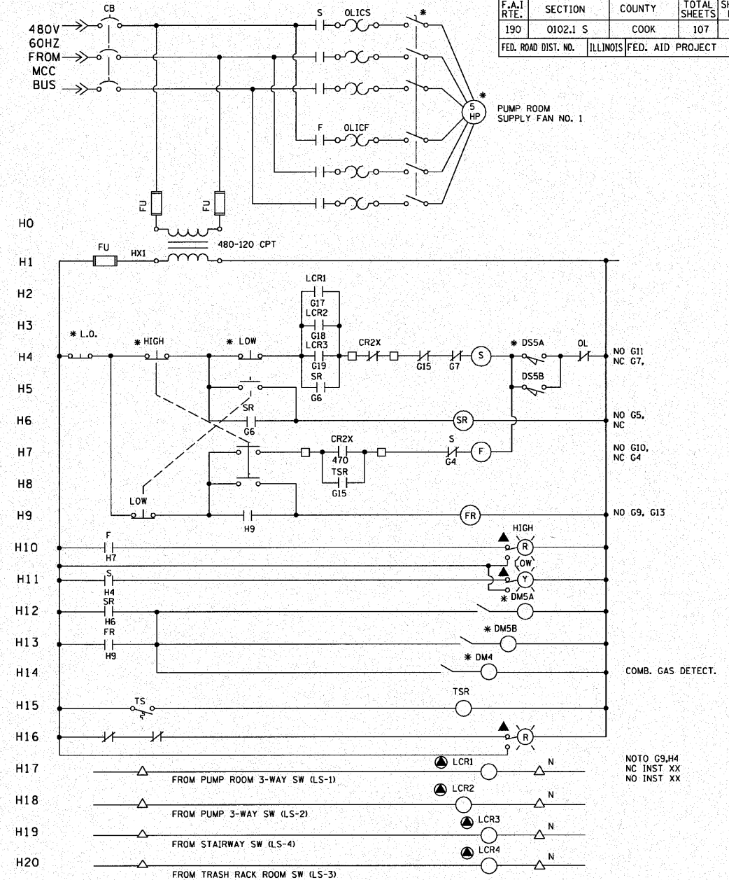
PUMP ROOM SUPPLY FAN SF-1
