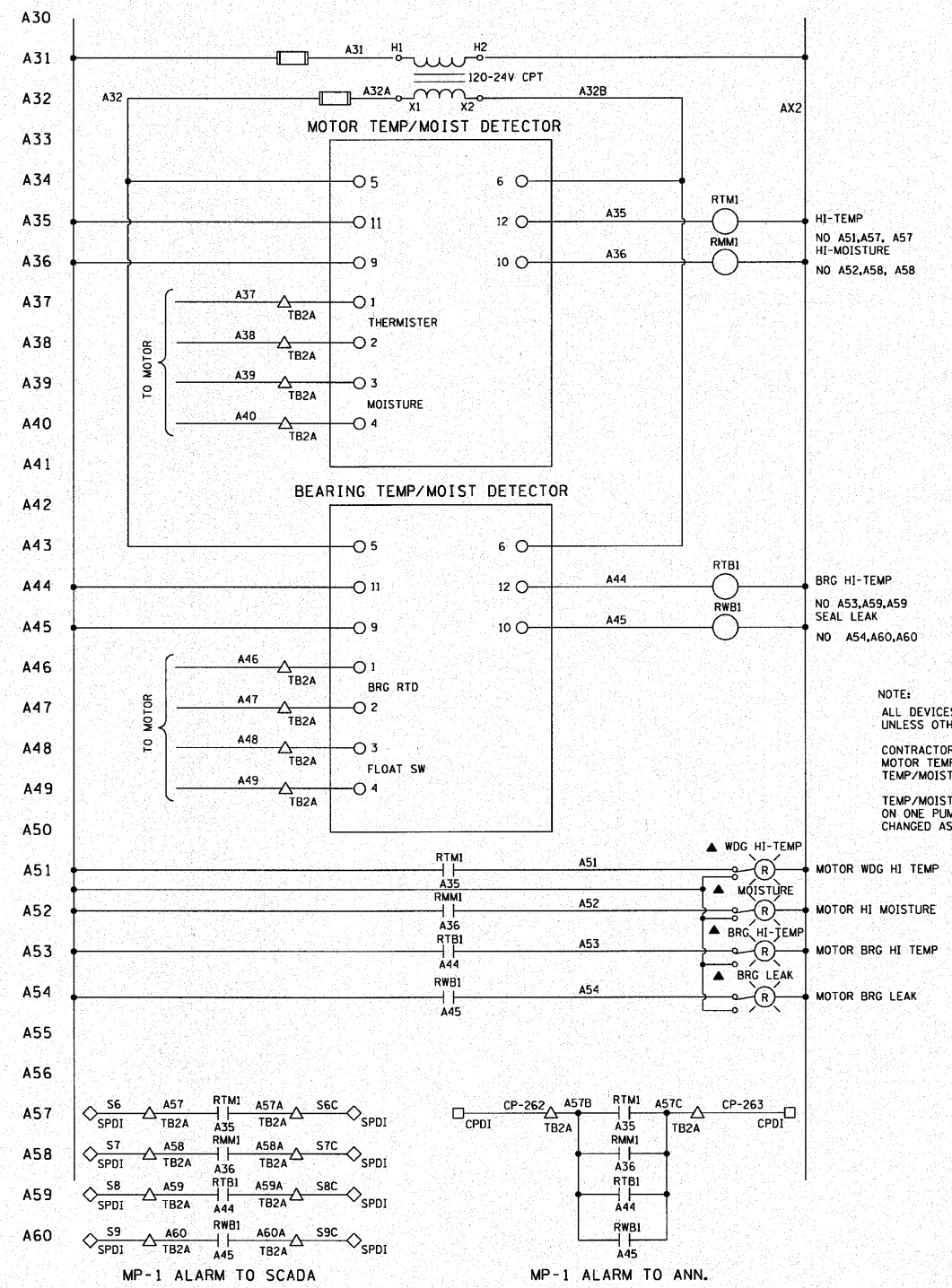
MAIN PUMP 1 CONTROL SCHEMATIC (TYPICAL FOR MAIN PUMPS 2, 3, 4, 5, 6 & 7)
