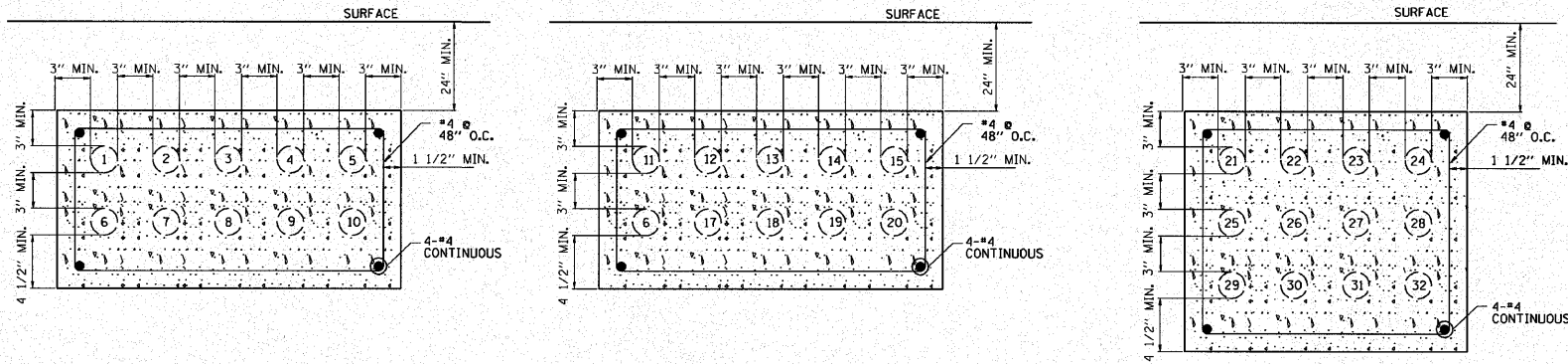
DUCT BANK SECTION A NTS E3
