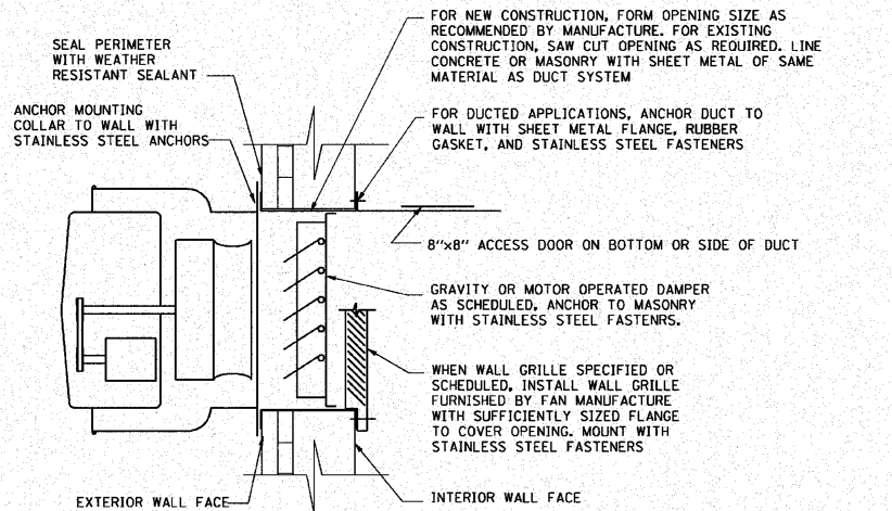
WALL MOUNTED EXHAUST FAN DETAIL
