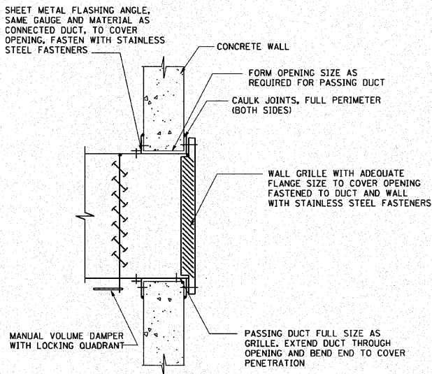
THROUGH WALL GRILLE DETAIL
