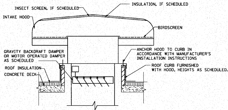
INTAKE HOOD ON ROOF CURB DETAIL
