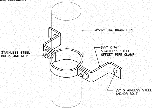
4" DIA. DRAIN PIPE SUPPORT
