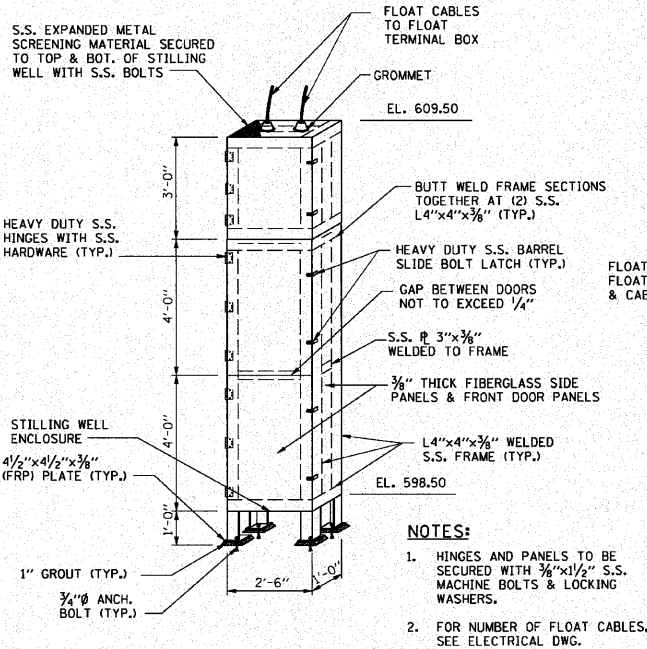
FLOAT STILLING WELL DETAIL FOR PUMP FLOAT CONTROL
