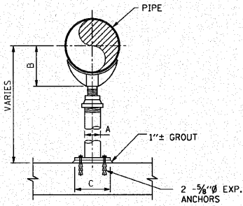
TYPICAL PIPE SUPPORT
