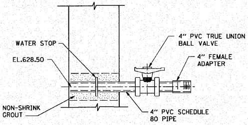
MAINTENANCE PUMP DISCHARGE PIPE DETAIL
