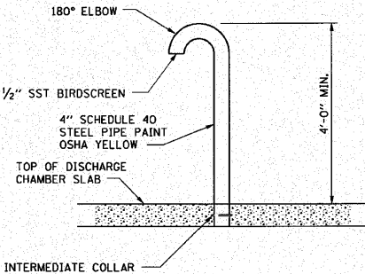
AIR VENT PIPE DETAIL
