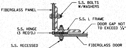
STAINLESS STEEL DOOR HINGE DETAIL
