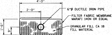
PIPE FOOTING DRAIN DETAIL
