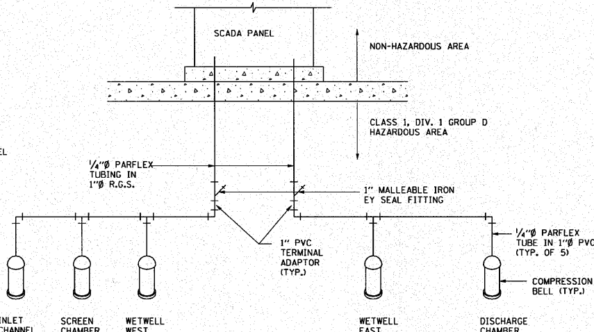
COMPRESSION BELL PIPING SCHEMATIC
