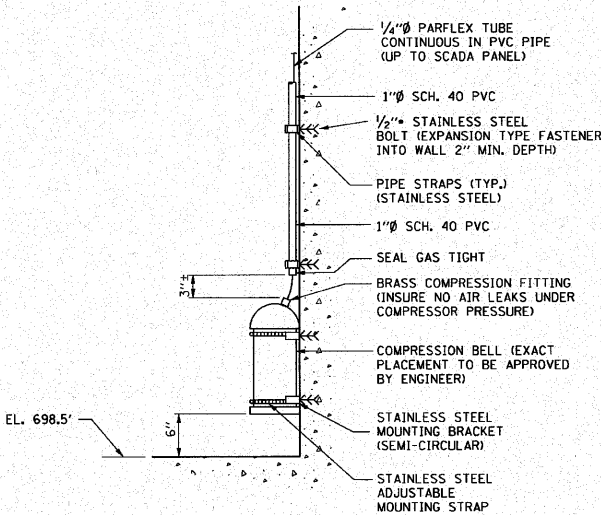
COMPRESSION BELL MOUNTING DETAIL
