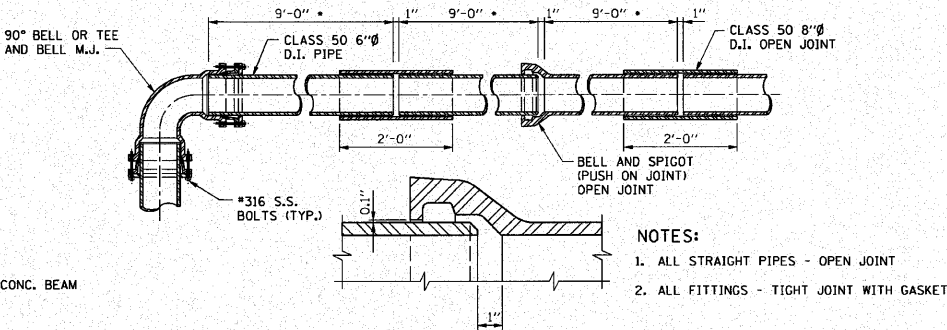
6" DIA. D.I. PIPE FOOTING DRAIN DETAIL
