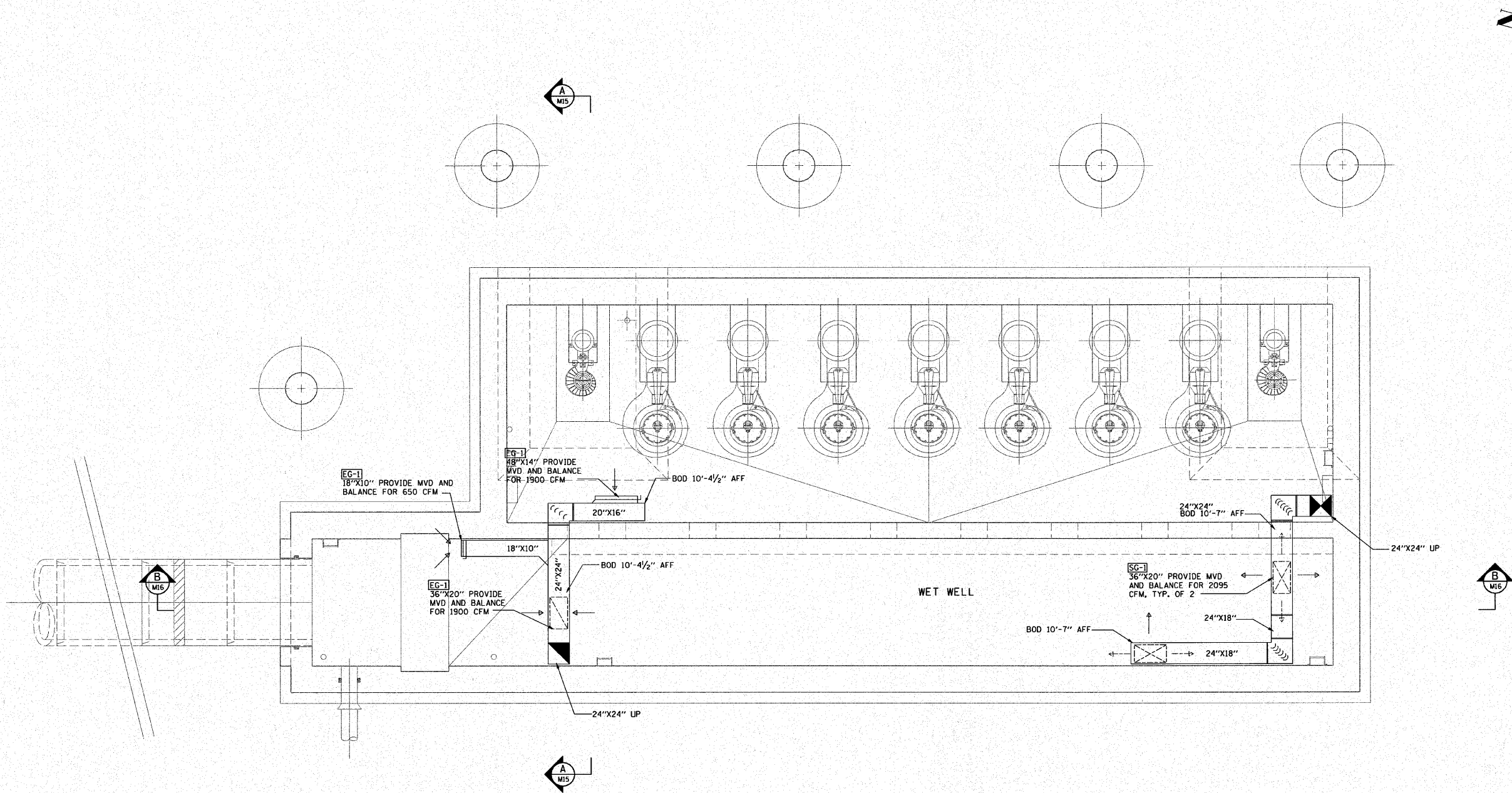
PLAN @ EL. 597.5
