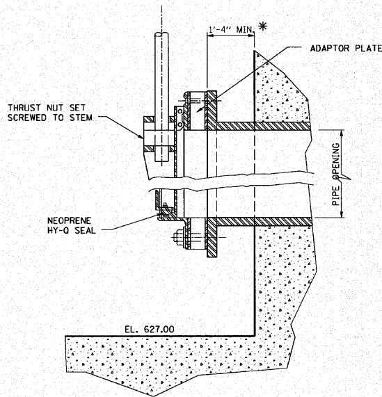
SECTION 3-3
