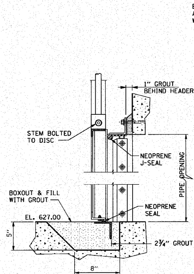
SECTION 1-1
