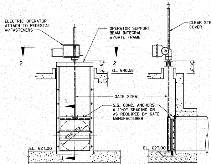
FRONT ELEVATION SIDE ELEVATION 84"x84" FLUSH BOTTOM SLIDE GATE DETAIL-S16 N.T.S.
