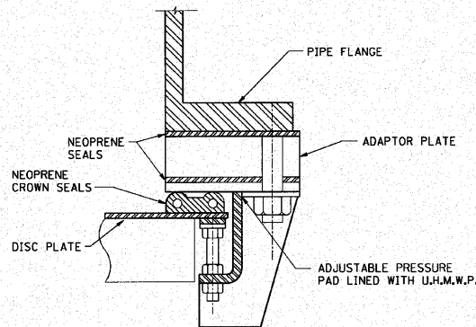
SECTION 4-4
