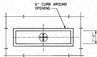
SECTION 2-2
