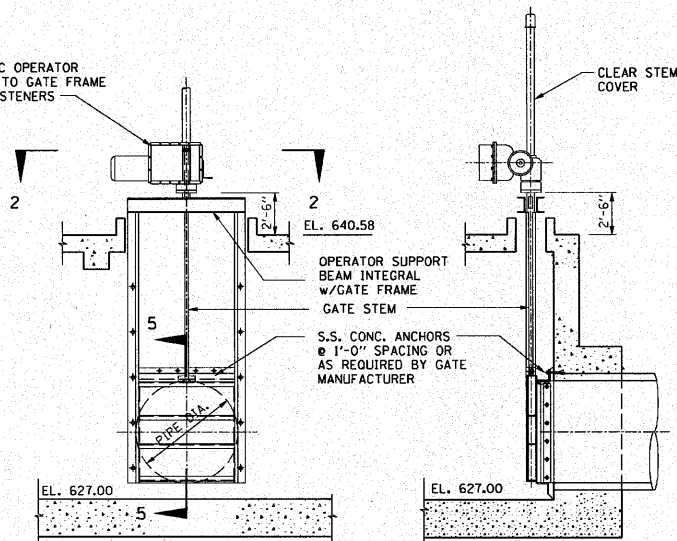
FRONT ELEVATION SIDE ELEVATION 72"x72" WALL MOUNTED INVERT SLIDE GATE DETAIL-S19 N.T.S.
