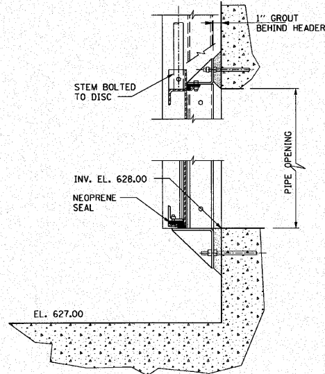
SECTION 5-5
