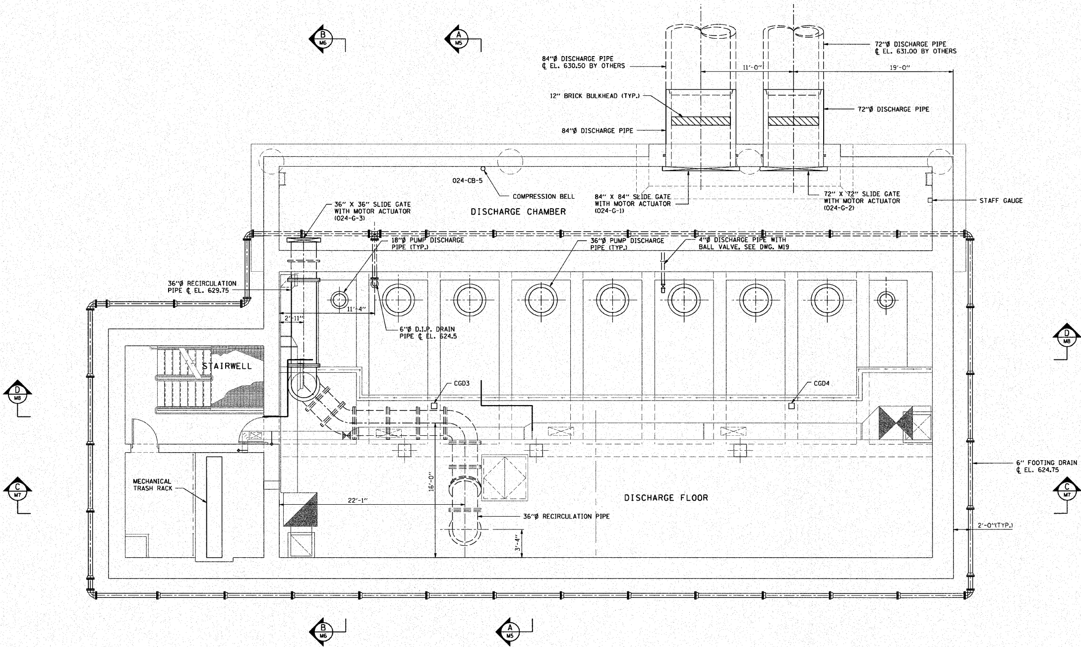
PLAN @ EL. 627.00
