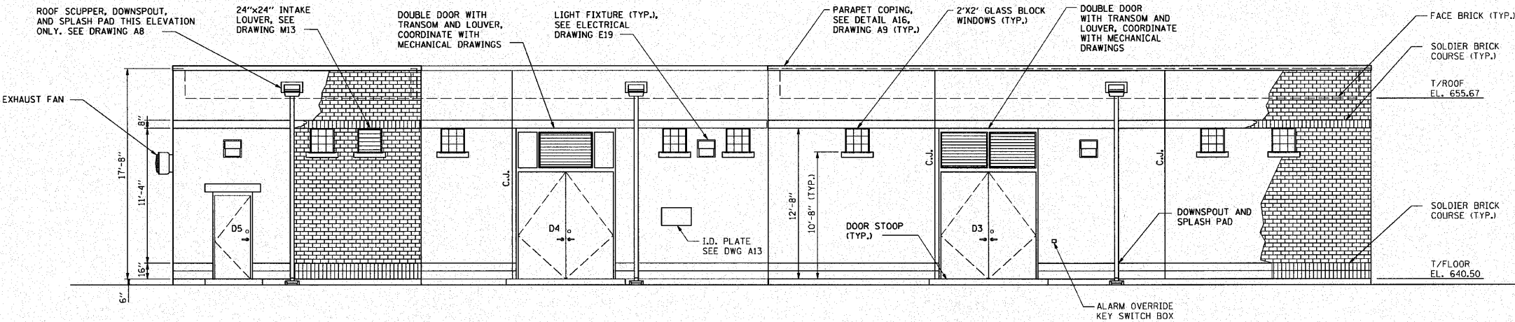
WEST ELEVATION
