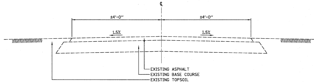
EXISTING TYPICAL CROSS SECTION STA 11+00.00 TO STA 14+50.00, FOX RIVER TRAIL
