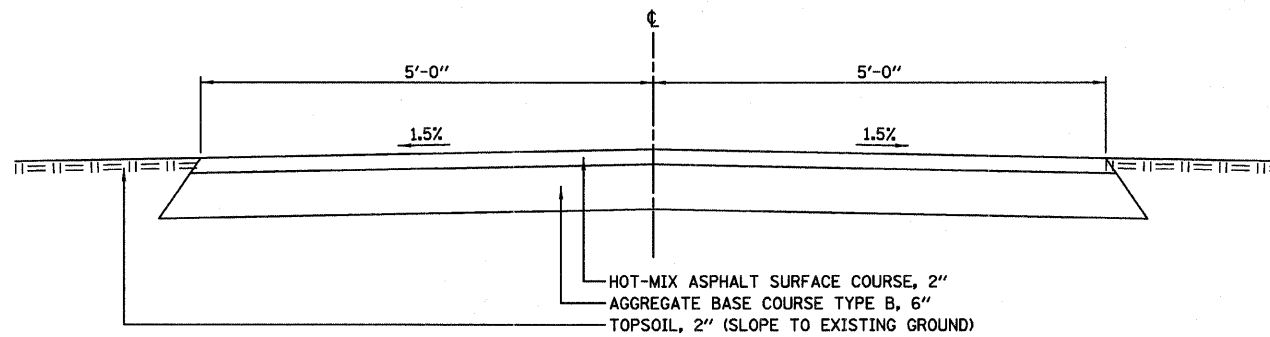
PROPOSED TYPICAL CROSS SECTION STA 11+00.00 TO STA 11+91.25, FOX RIVER TRAIL STA 13+92.75 TO STA 14+50.00, FOX RIVER TRAIL
