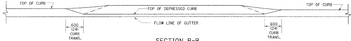
SECTION B-B
