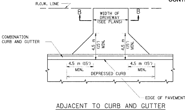
ADJACENT TO CURB AND GUTTER
