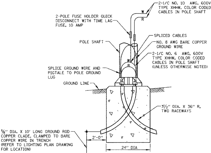
POLE BASE WIRING DETAIL
