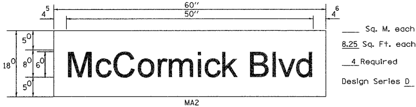
PANEL SIGN DESIGN TYPE 2
