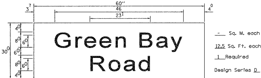
PANEL SIGN DESIGN TYPE 2
