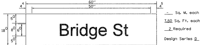
PANEL SIGN DESIGN TYPE 1
