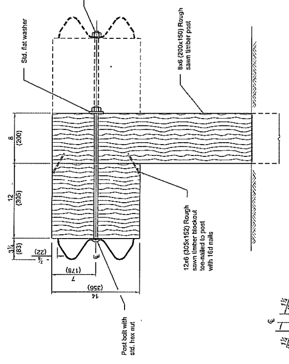
WOOD POST CONSTRUCTION
