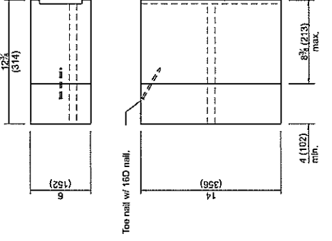
TWO-PIECE WOOD BLOCKOUT OPTION
