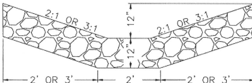
DETAIL OF AGGREGATE DITCH (SPECIAL)
