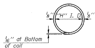
PLAN-COIL WIRE
