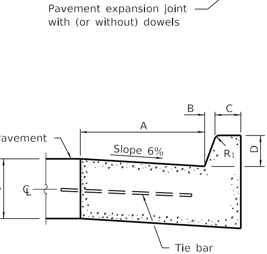
BARRIER CURB
