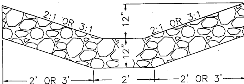
DETAIL OF AGGREGATE DITCH (SPECIAL)
