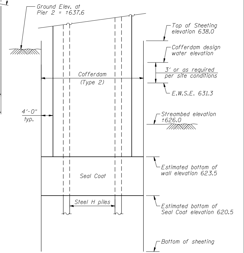
SEAL COAT SCHEMATIC (Required at Pier 2 only)
