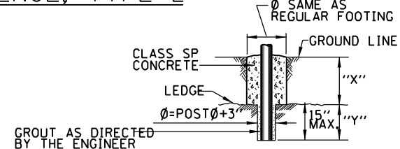
FOOTING FOR POST WHEN ROCK LEDGE IS ENCOUNTERED
