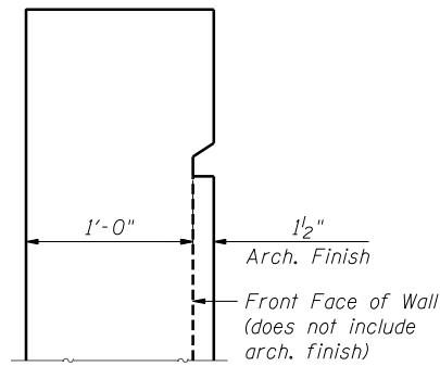
DETAIL 1
