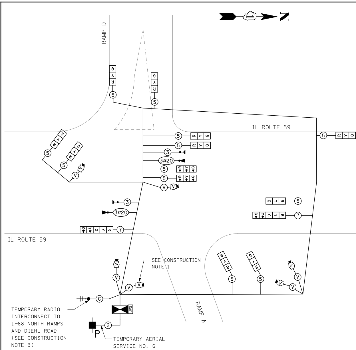
TEMPORARY SIGNAL CABLE PLAN STAGE 3B
