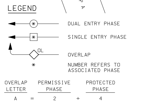
TEMPORARY PHASE DESIGNATION DIAGRAM STAGE 3B
