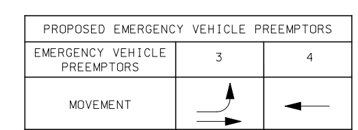
EMERGENCY VEHICLE PREEMPTION SEQUENCE STAGE 2
