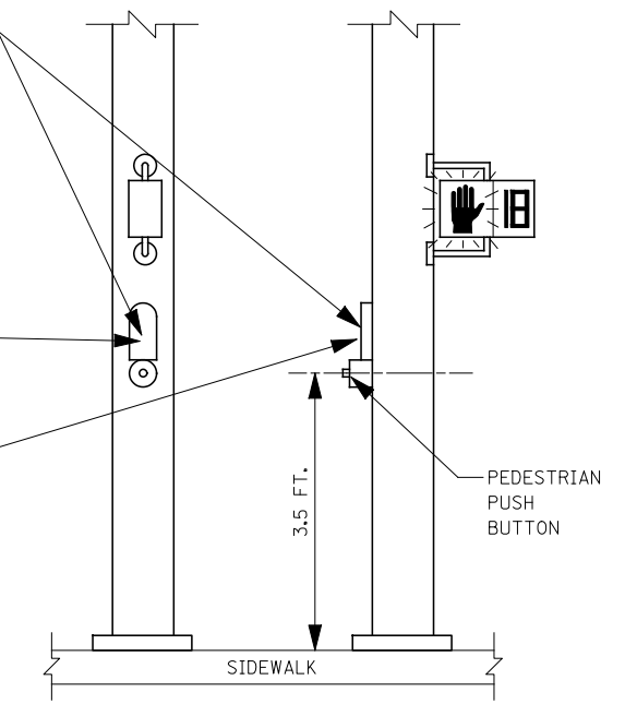
PEDESTRIAN PUSH BUTTON SIGN MOUNT DETAIL NOT TO SCALE
