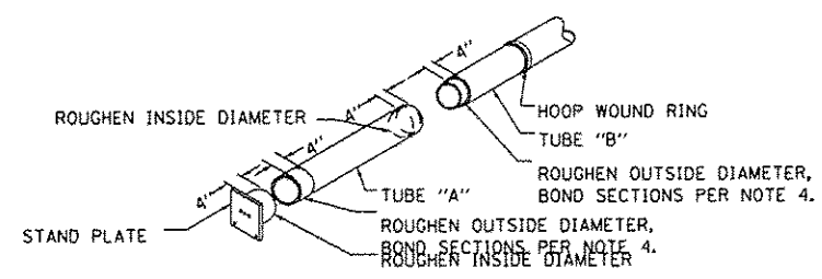
DETAIL 3 LIR TUBE ASSEMBLY DETAILS
