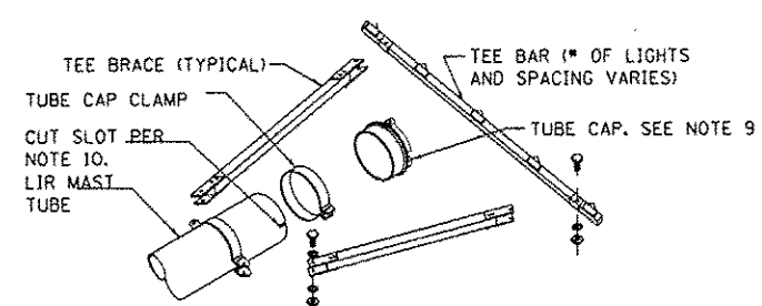
DETAIL 5 TEE BRACE ASSEMBLY DETAILS
