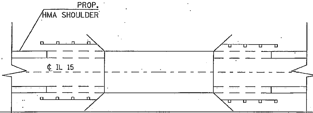
TYPICAL EXISTING HMA SHOULDERS @ STRUCTURES
