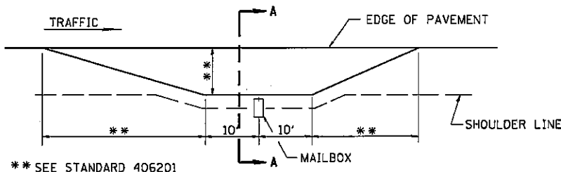
PLAN AT PRIVATE & COMMERCIAL ENTRANCES
