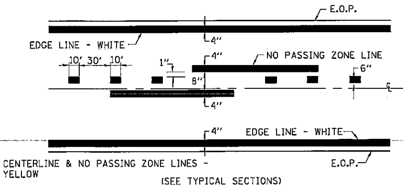
PAVEMENT MARKING
