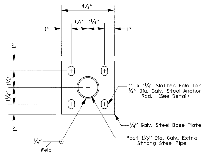
POST BASE PLATE DETAIL
