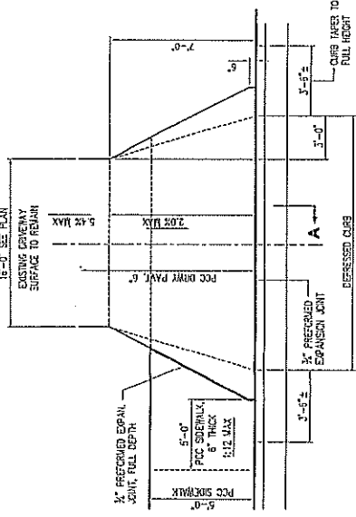
PRIVATE ENTRANCE PLAN EAST SIDE OF WIGWAM HOLLOW ROAD
