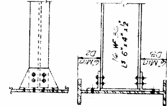
DIAPHRAGM D2 & D3 SERIES 203 Required
