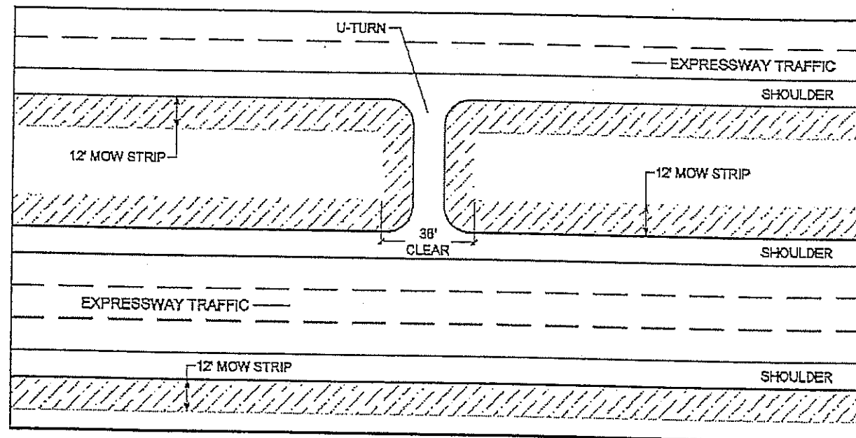
Mowing Detail #5
