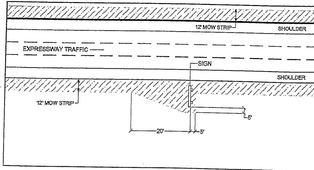
Mowing Detail #4
