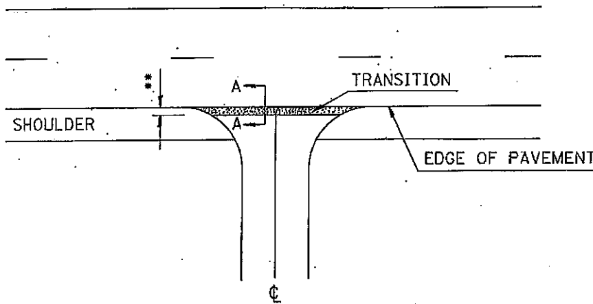
SIDEROAD DETAIL
