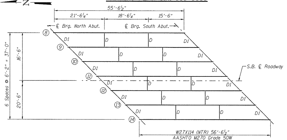
FRAMING PLAN S.N. 068-0039
