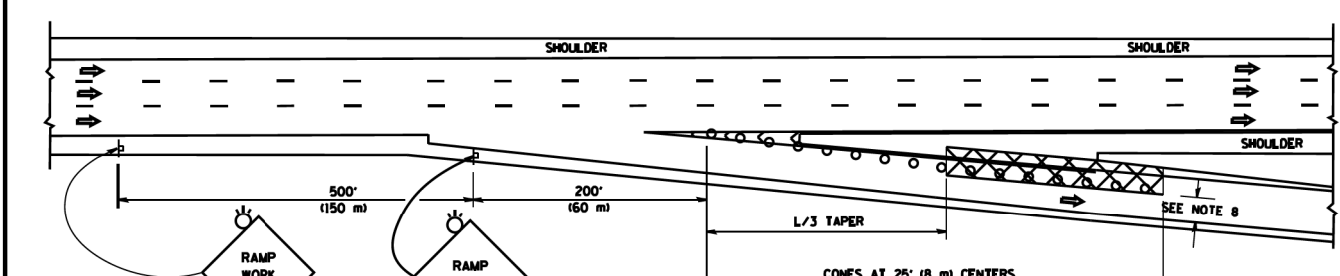
TYPICAL EXIT RAMP
