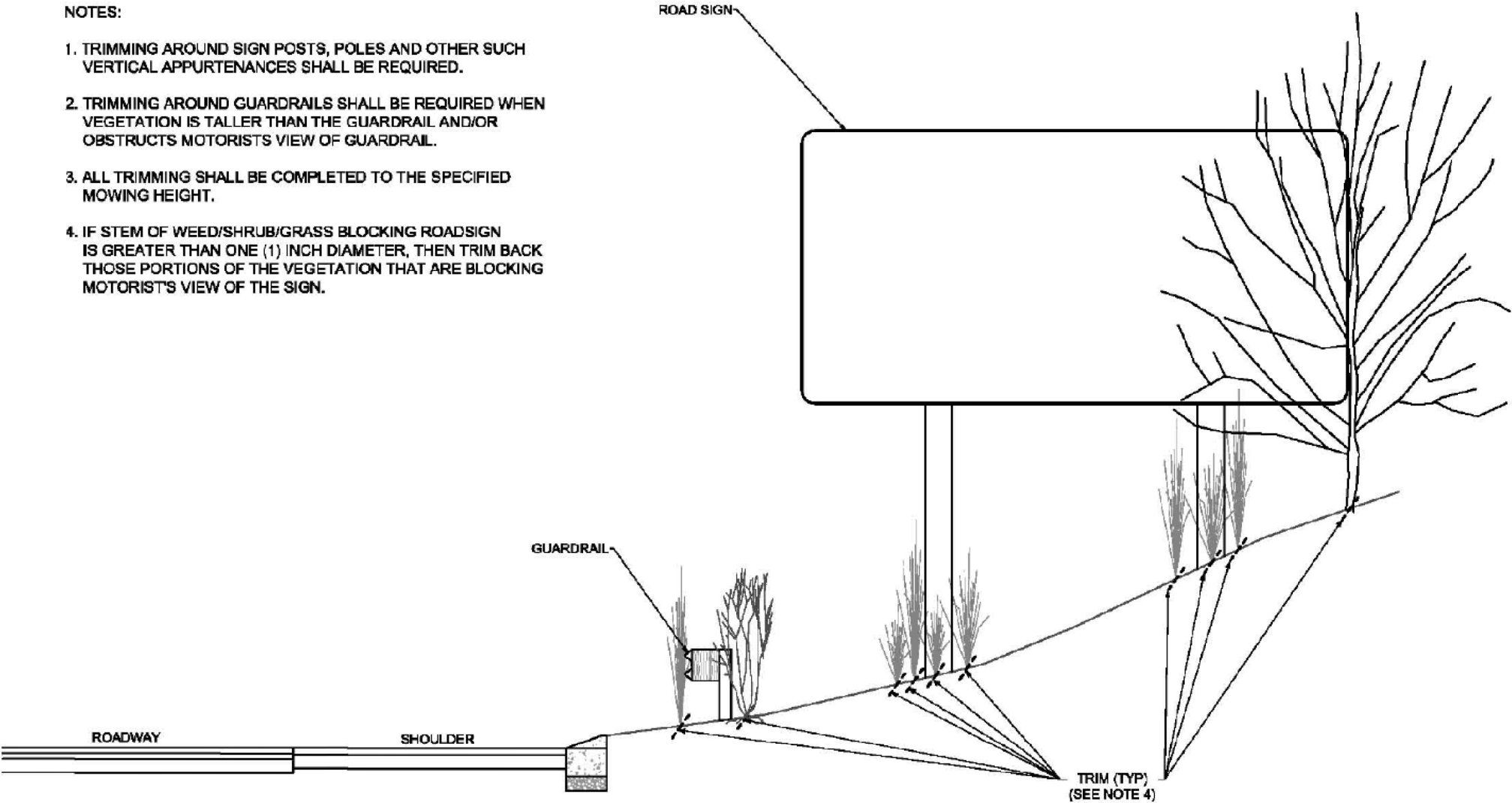
Trimming Detail Not to Scale
