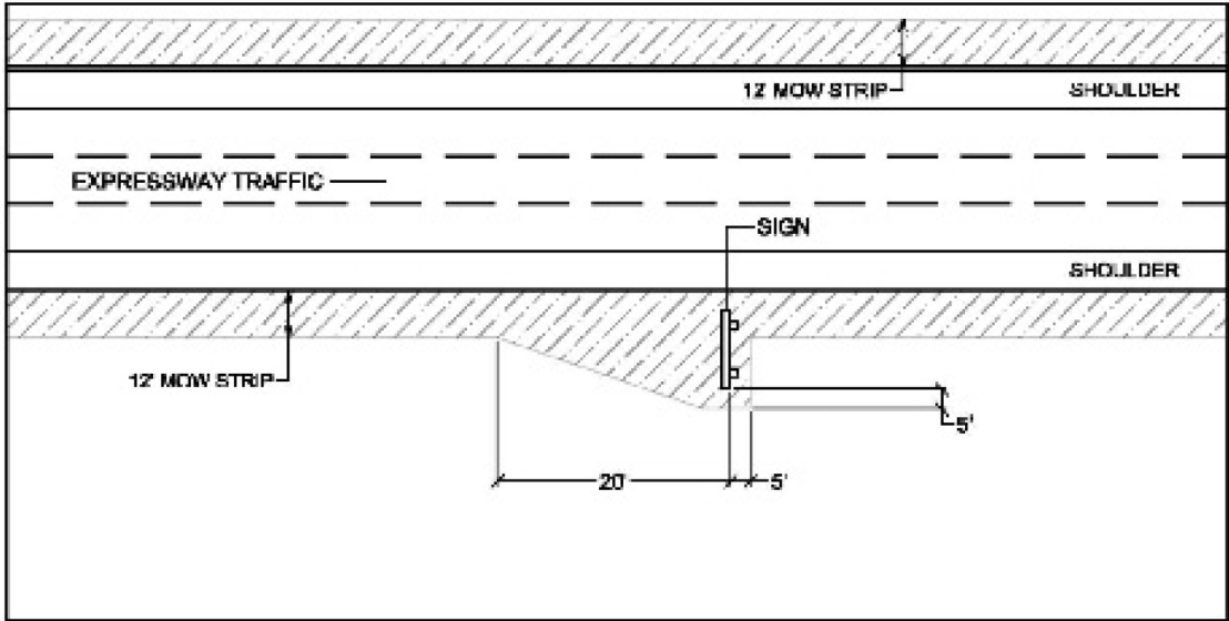
Mowing Detail #4 Not to Scale Roadway Signs
