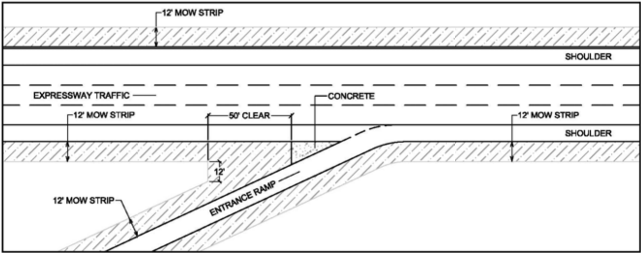
Mowing Detail #3
