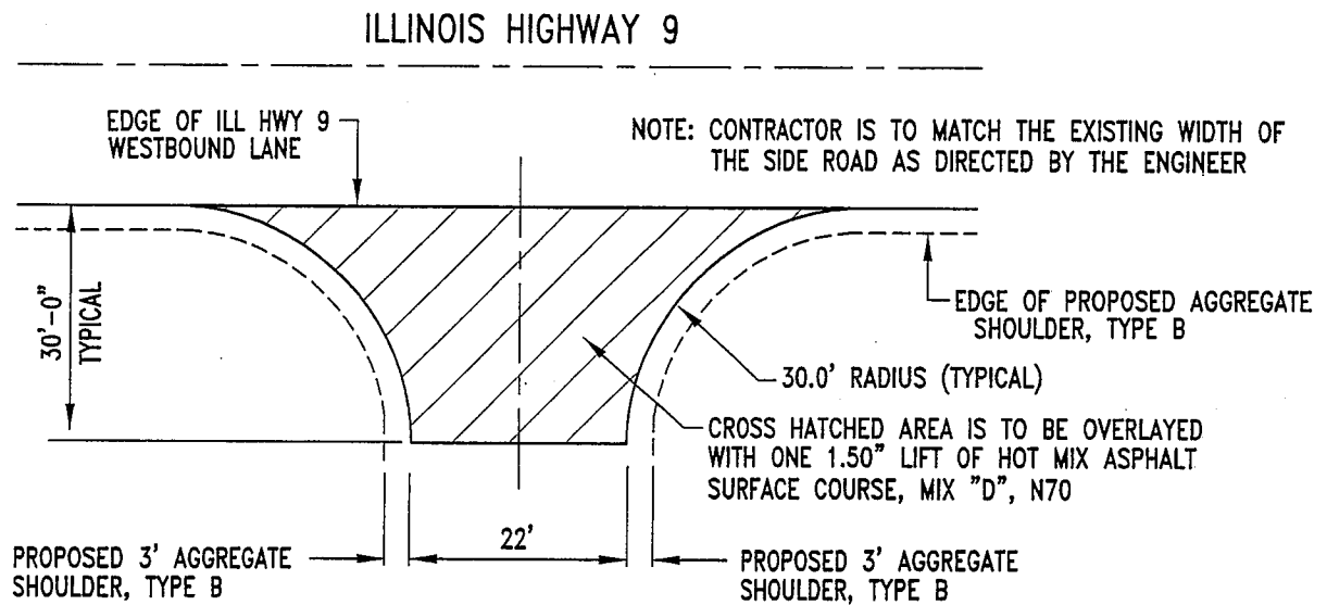
TYPICAL PLAN VIEW OF INTERSECTION AT ILL HWY 9
