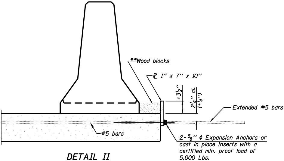
DETAIL II
