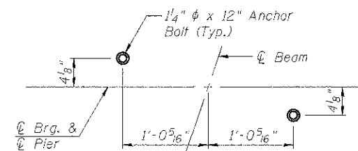
ANCHOR BOLT LOCATION DETAIL
