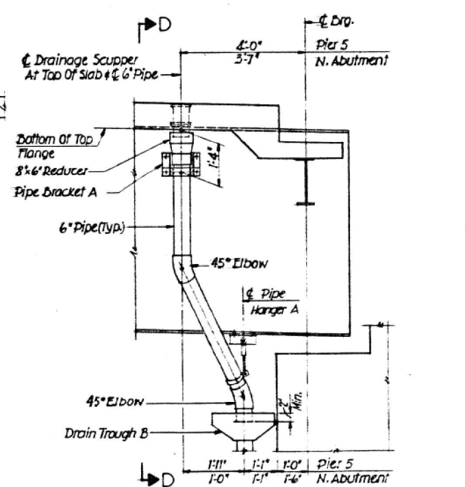
ELEVATION AT PIER 5 ELEVATION AT N. ABUT. OPP. HAND
