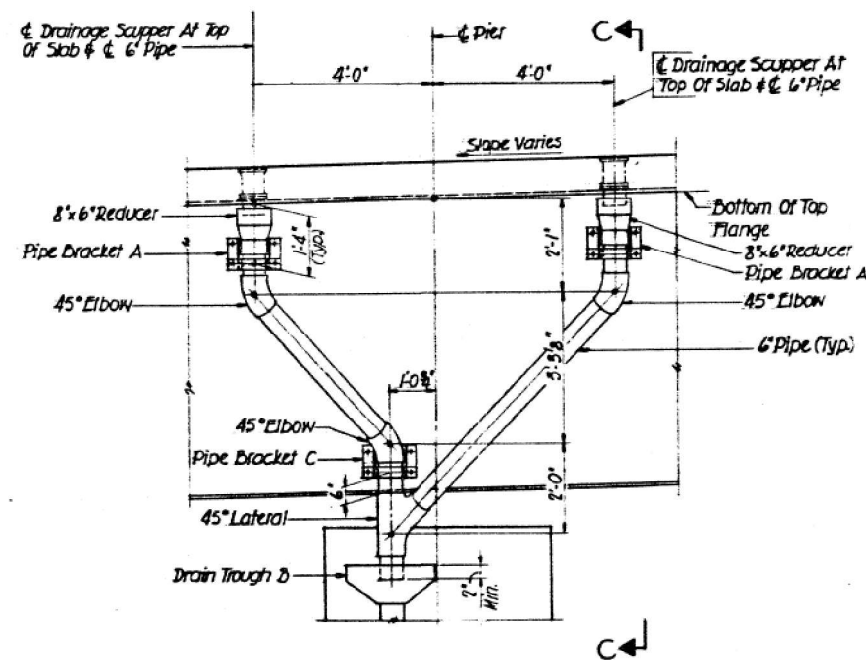
ELEVATION AT PIERS 6 THRU 15
