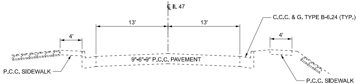
EXISTING TYPICAL SECTION 3 L.M. 3.87 TO L.M. 4.02
