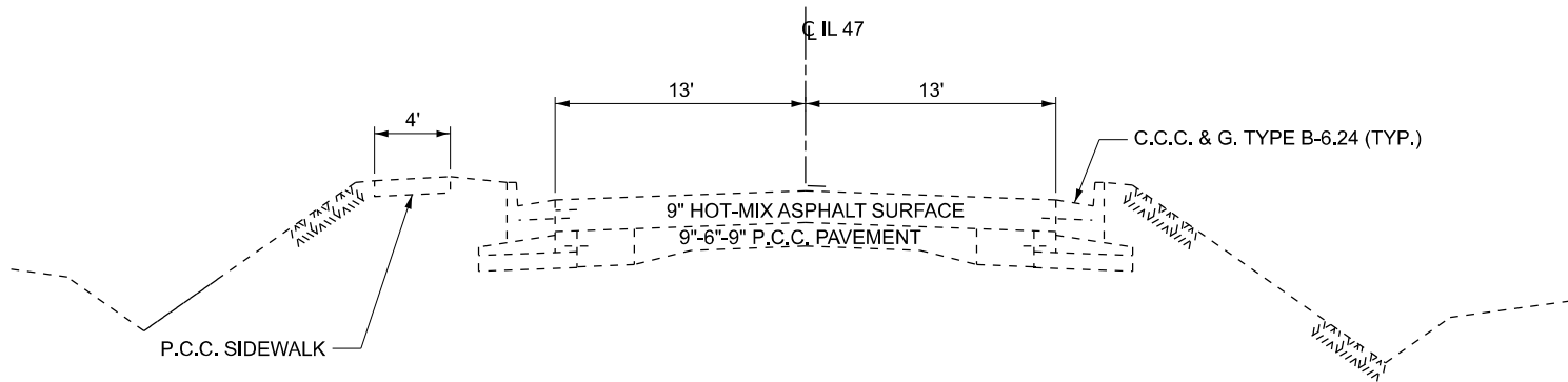
EXISTING TYPICAL SECTION 2 L.M. 3.47 TO L.M. 3.87
