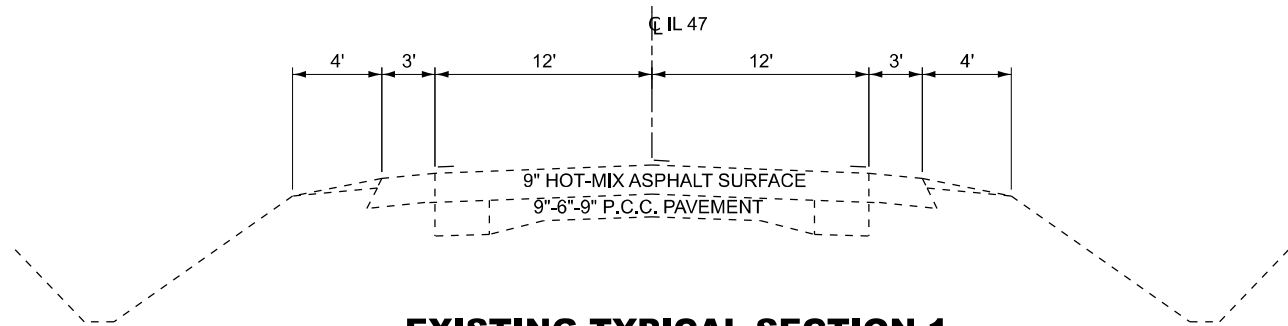
EXISTING TYPICAL SECTION 1 L.M. 0.00 TO L.M. 3.47
