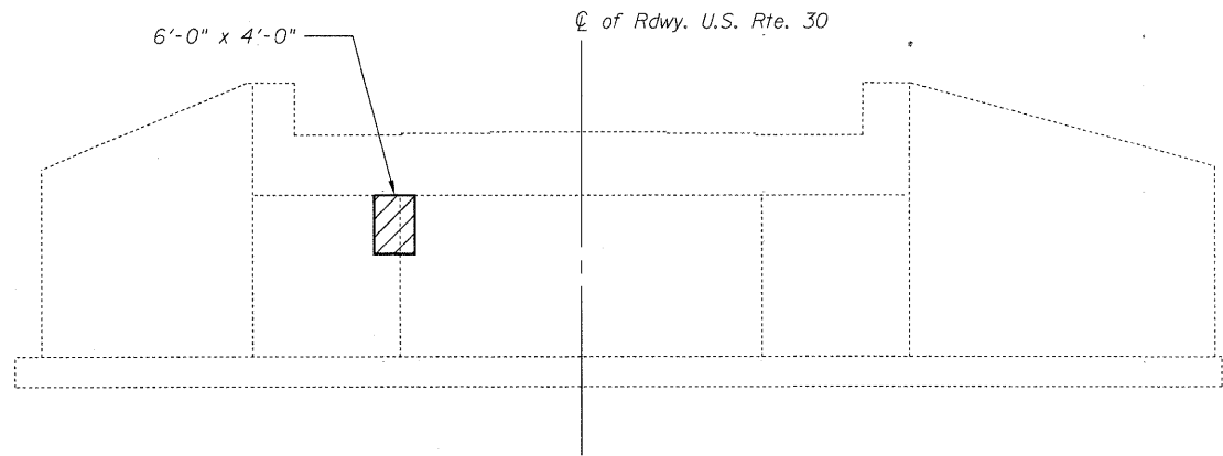
ELEVATION - WEST ABUTMENT
